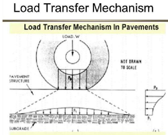
Figure 4 : Load transfer in rigid pavement
