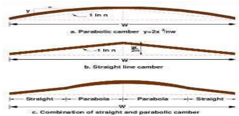
Figure : Different types of camber
