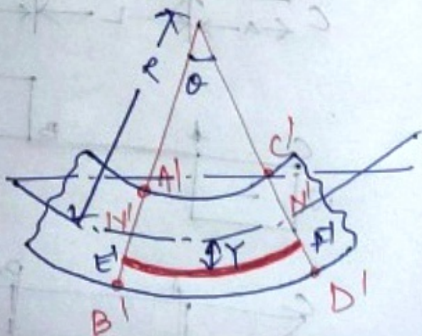
After Bending
